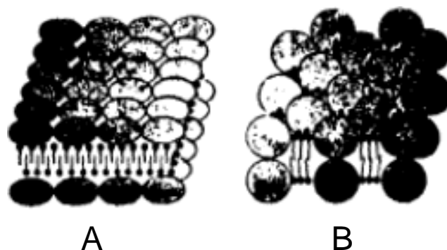
FIGURE 6. (A) Davson-Danisili model for structure of biological membranes. (B) Lipid-protein mosaic model for the structure of biological membranes.
