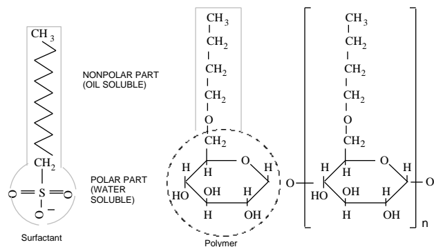
FIGURE 2. The structure of surface-active molecules. The broken line shows the separation of polar and non-polar parts of the molecule.
