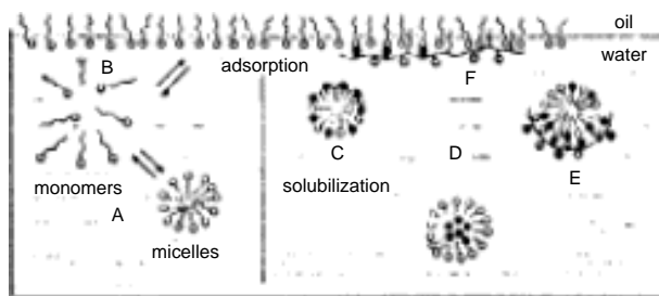
FIGURE 3. A schematic presentation of adsorption, micelle formation, and solubilization processes in surfactant solutions.
