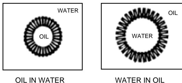
FIGURE 8. A schematic presentation for the structure of emulsion droplets and orientation of surface-active molecules at the oil-water interface.
