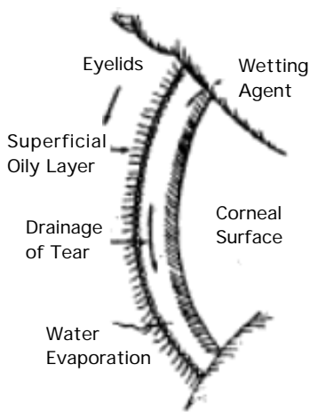
FIGURE 14: A schematic presentation of various surface phenomena occurring in the eye.
