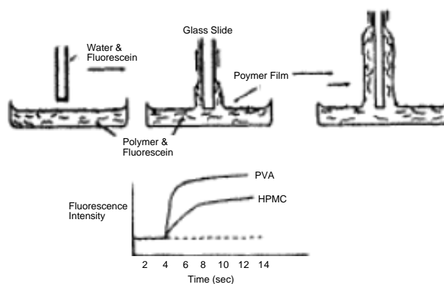
FIGURE 16. The slide technique used to measure the thickness of water layer dragged with a moving polymer film.
