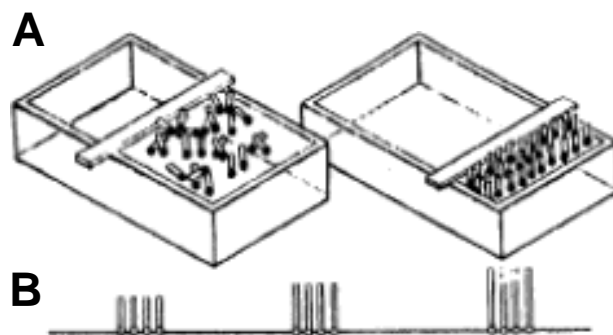
FIGURE 5. (A) schematic illustration of a monomolecular film at air/water interface. (B) Orientation of surface-active molecules with increasing chain-length at air-water interface.
