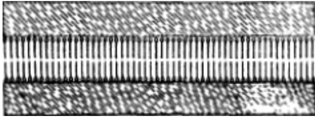
FIGURE 9. A schematic presentation of the orientation of surface-active molecules at the metal surface in boundary lubrication.
