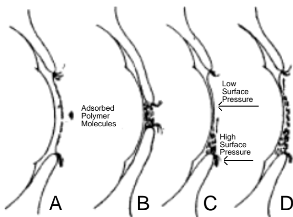
FIGURE 15. A schematic presentation of the effect of adsorbed polymer film at the air-tear interface in upward movement of water after a blink.
