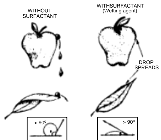
FIGURE 10. A schematic presentation of the role of contact angle and wettability in influencing the effectiveness of agricultural sprays.
